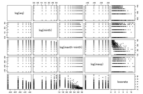
図3 REDのパケット棄却率に関する多変量相関図 (変数変換後) Fig. 3 Pair scatter plot of control parameters and packet loss probability (with variable transformation)
